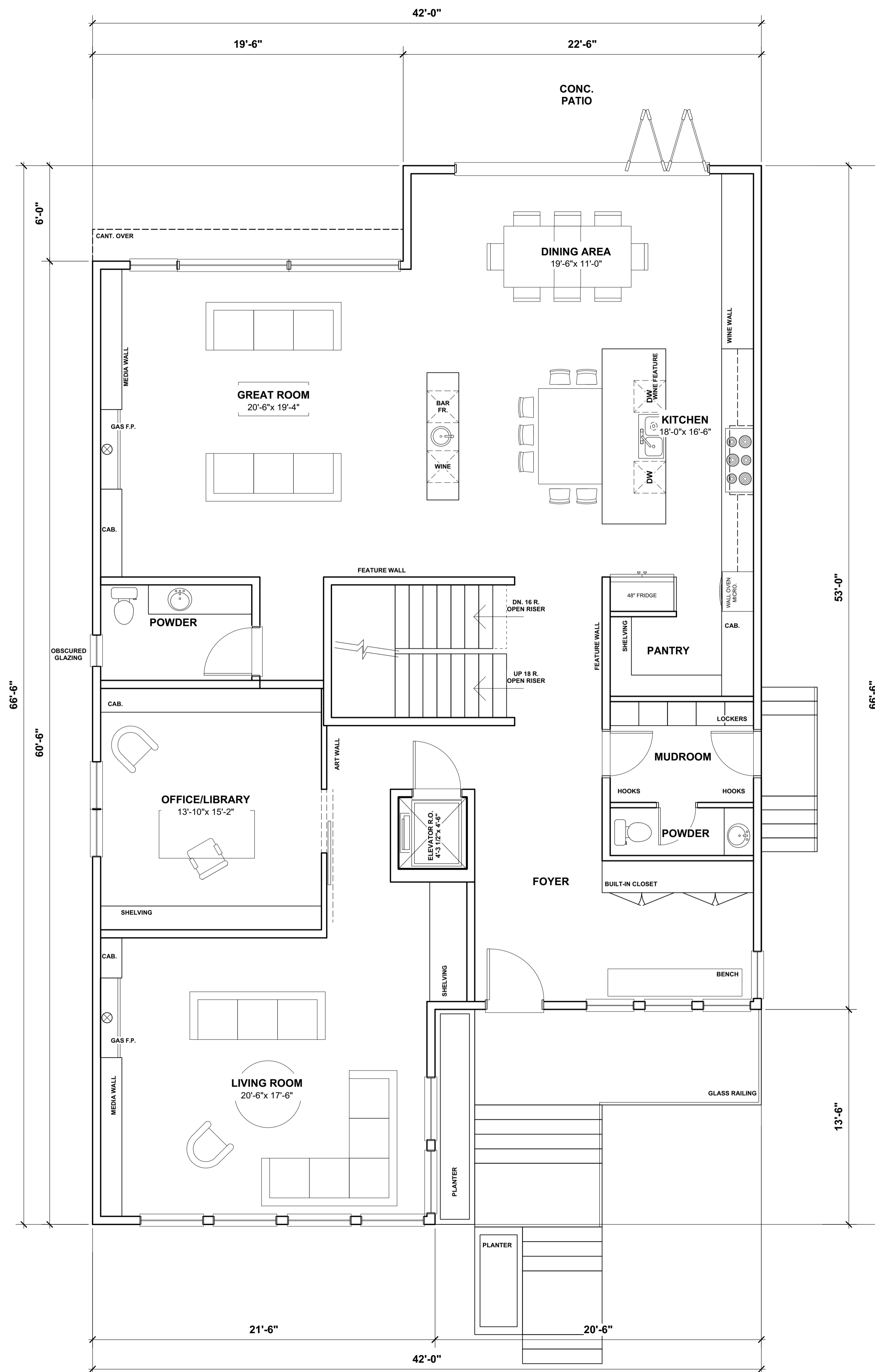
1 MAIN FLOOR PLAN A3 SCALE 1/4" = 1'-0" 2468 sq.ft.
